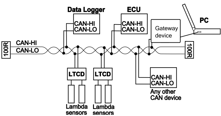
Wiring example
