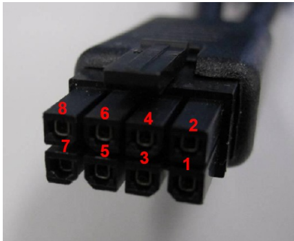
8 Pin Micro-Fit
